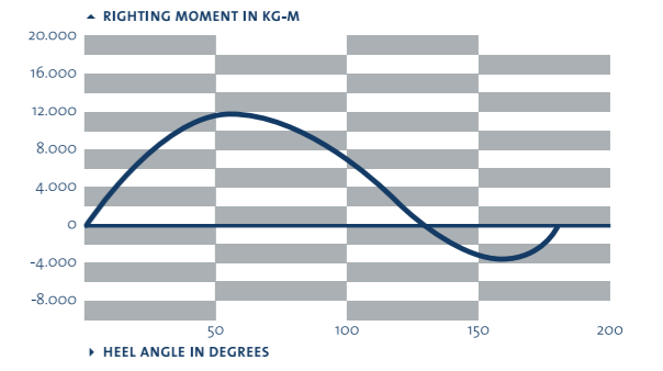
STABILITY CURVE
