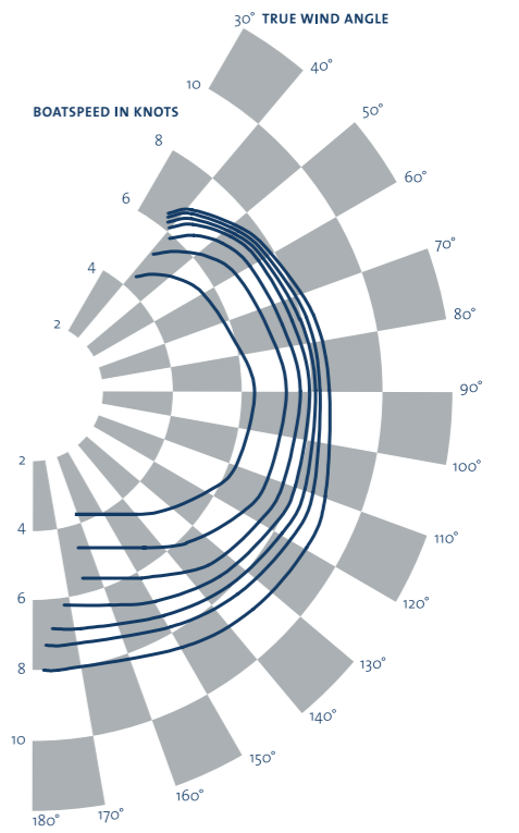
POLAR PERFORMANCE DIAGRAM
