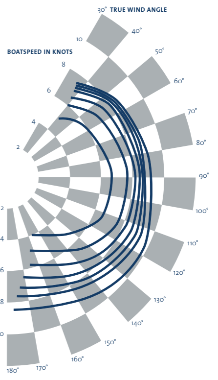
POLAR PERFORMANCE DIAGRAM
