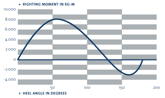
STABILITY CURVE
